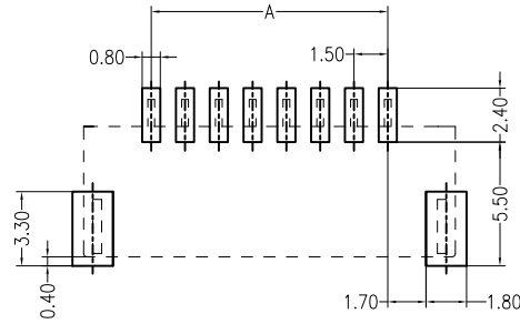
PCB LAYOUT(Tolerance:±0.05)
