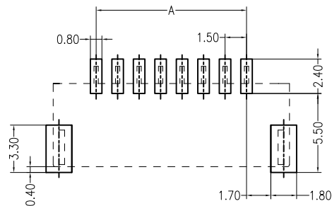
PCB LAYOUT(Tolerance:±0.05)
