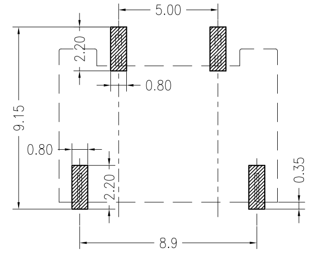
Board Layout
