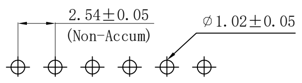
PCB LAYOUT
