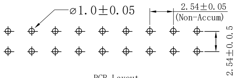
PCB Layout
