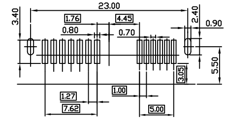
RECOMMENDED P.C.B LAYOUT TOLERANCES±0.05(TOP VIEW)
