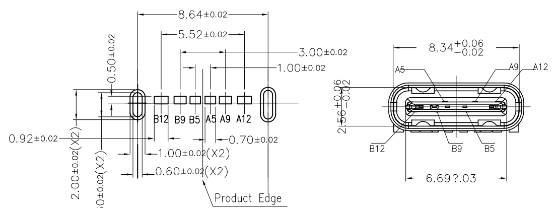
RECOMMENDED P.C.B. LAYOUT TOLERANCE UNSPECIFIED ±0.05mm
