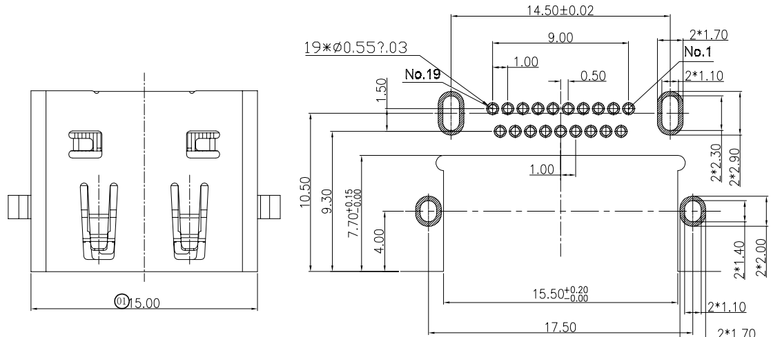
Recommended pcb layout (top view) (thickness=1.2±0.10mm) (tolerance ±0.05)
