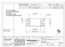
Technical drawing 14.0155
