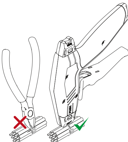
HellermannTyton plastic ties inside and outside serrated
