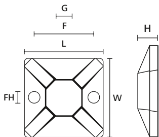
MB3-MB5 (plan view)
