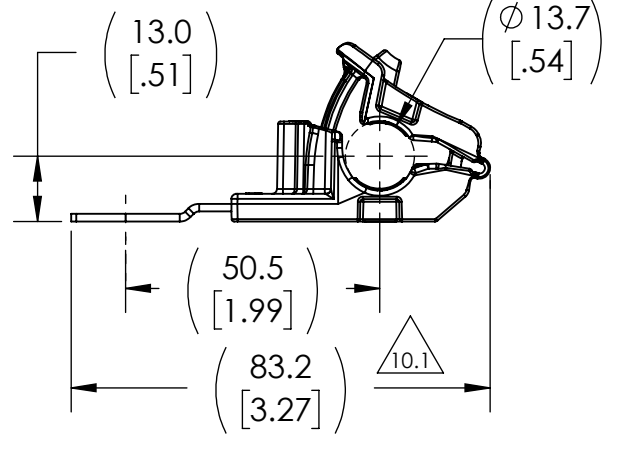
CONFIGURATION: 1
