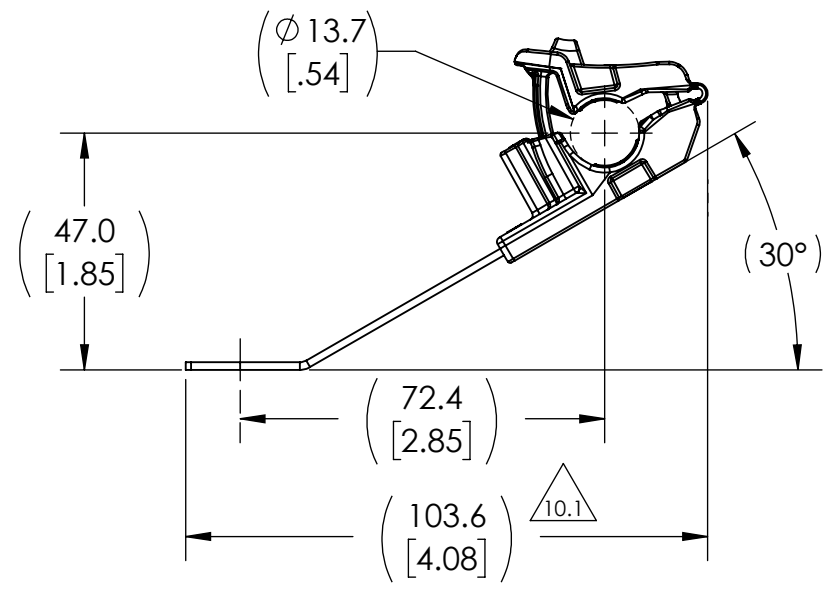
CONFIGURATION: 6
