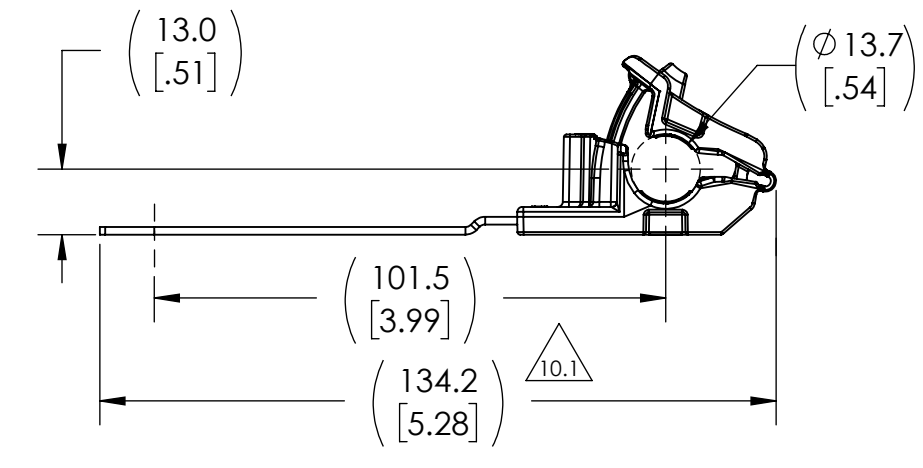
CONFIGURATION: 3
