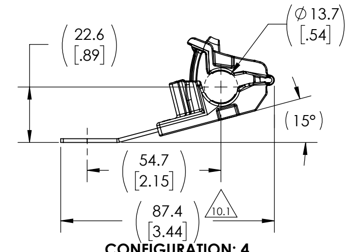
CONFIGURATION: 4
