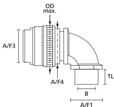
HeliaGuard compression fitting, 90° with fixed external thread
