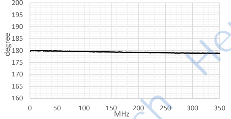
Phase Balance
