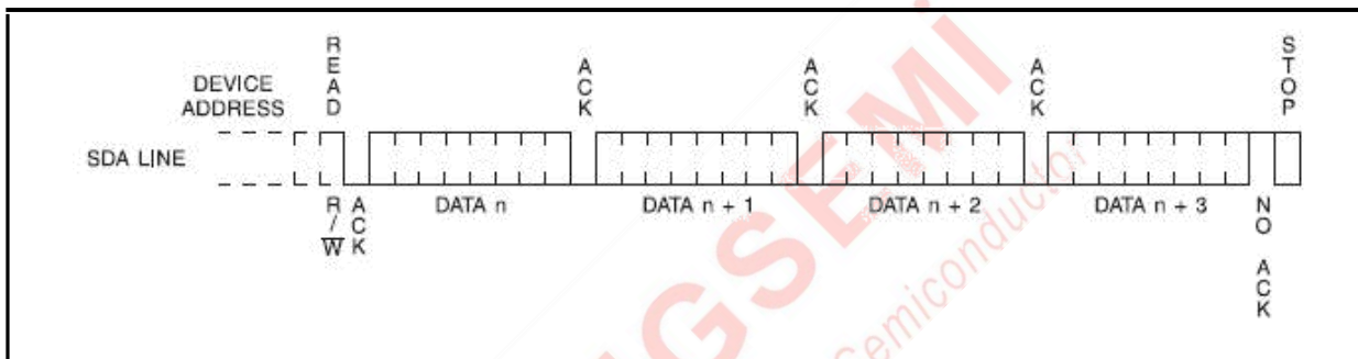
Figure 9. Sequential Read
