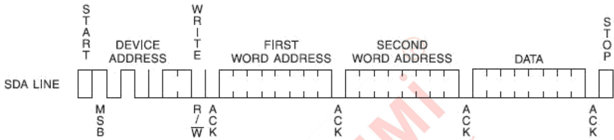
Figure 5. Byte Write
