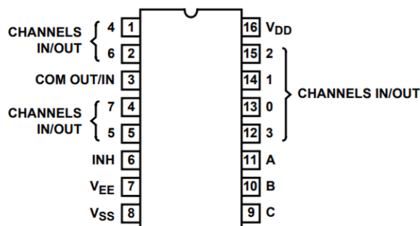
DIP16/SOP16/TSSOP16
