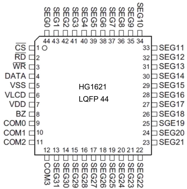
HG-1621BQ LQFP-44
