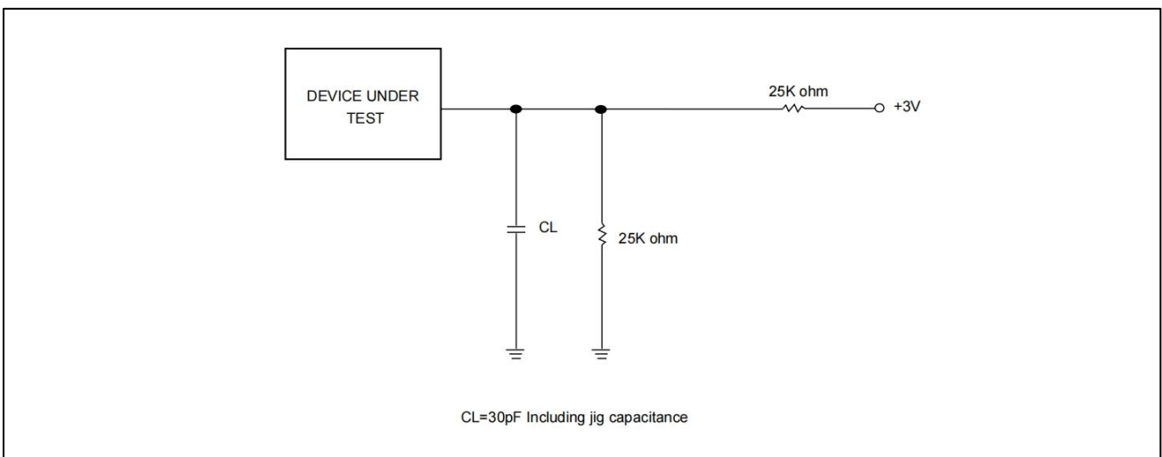
Figure 88. OUTPUT LOADING
