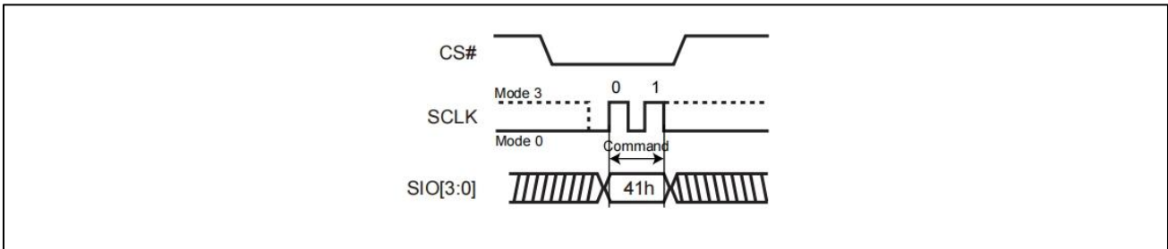
Figure 13. Factory Mode Enable (FMEN) Sequence (QPI Mode)
