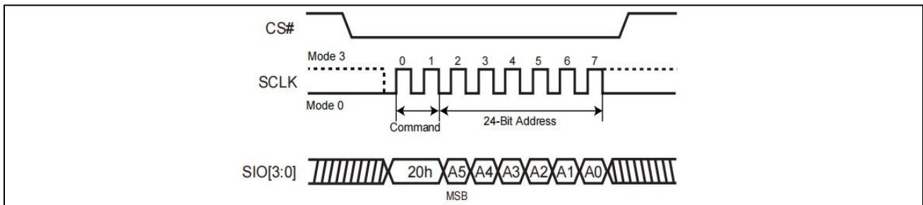
Figure 51. Sector Erase (SE) Sequence (QPI Mode)
