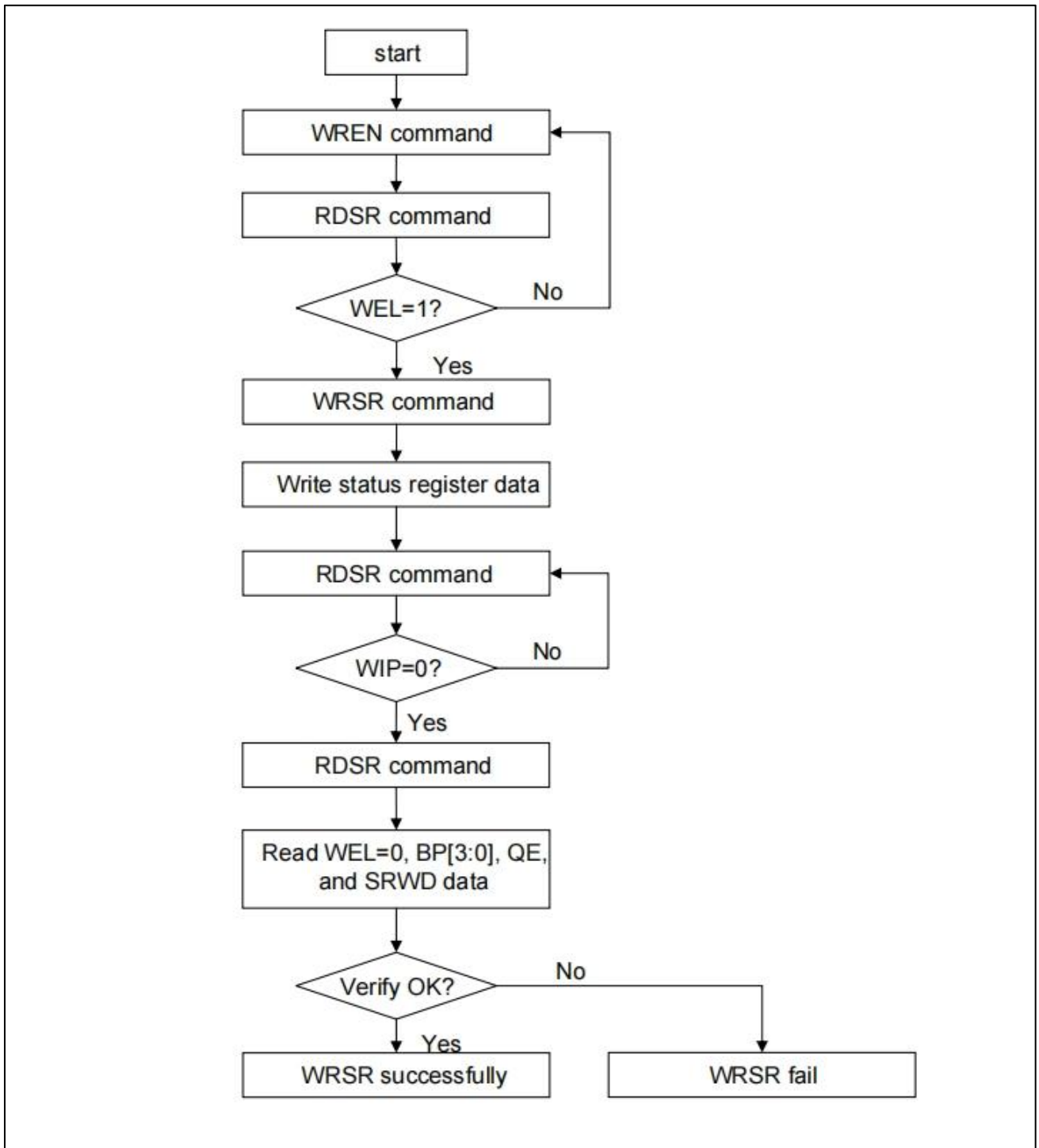
Figure 28. WRSR flow
