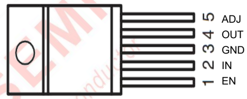
TO220-5
