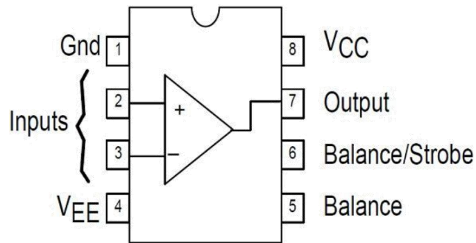
DIP8/SOP8/MSOP
