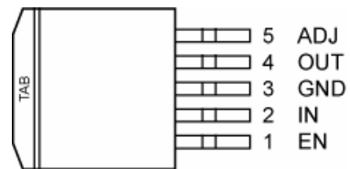
5-Pin TO-263 (D 2 Pak) Adjustable Voltage (U) LM29302/29502
