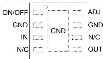
8-Lead LLP Surface Mount Package
