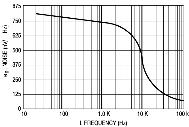
Figure 6. Noise Voltage
