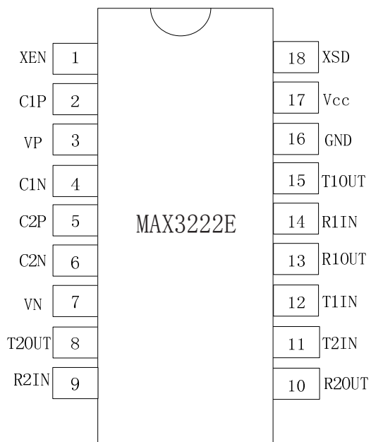
18-pin WSOIC
