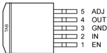
5-Pin TO-263 (D 2 Pak) Adjustable Voltage
