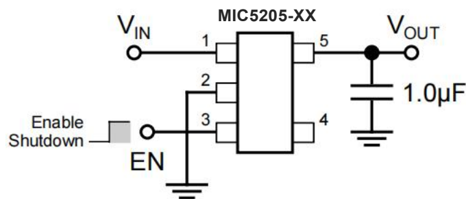
Figure 2. Low-Noise Fixed Voltage Application
