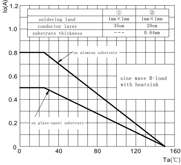
FIG1:Io-Ta Curve
