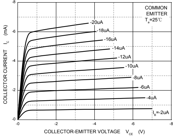
Static Characteristic
