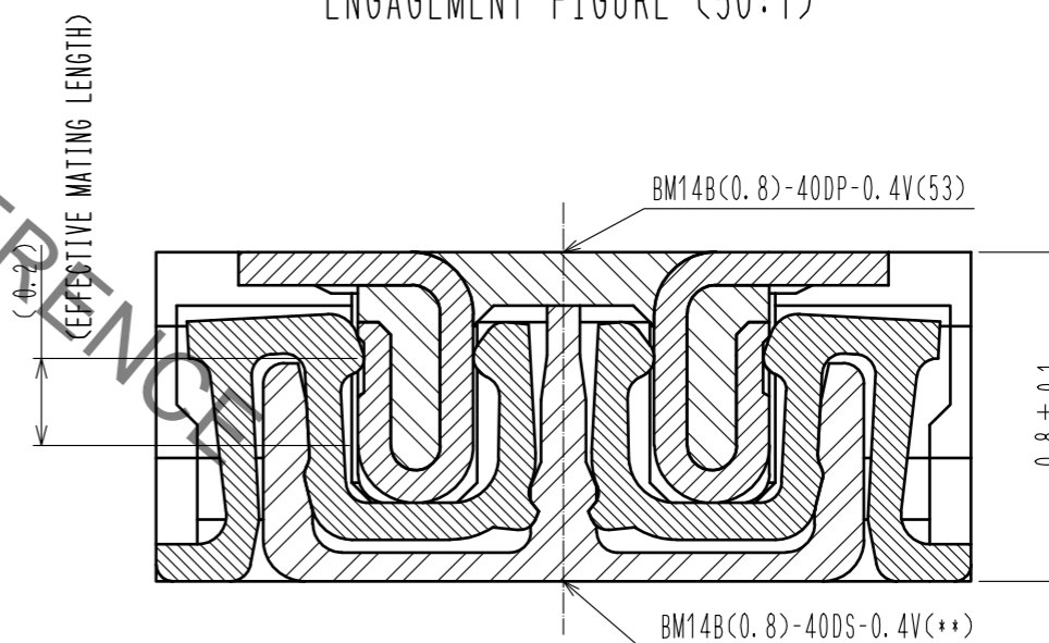
ENGAGEMENT FIGURE (50:1)
