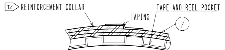
E-E (FREE)
