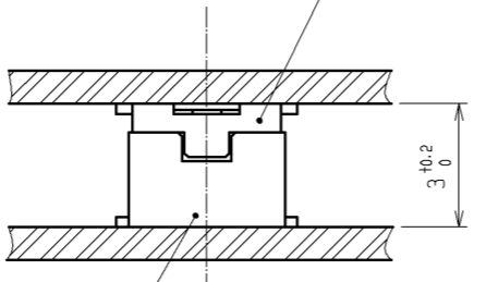
DF12E(3.0)-14DP-0.5V(81)
