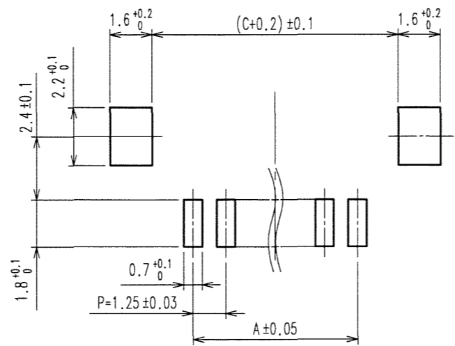
RECOMMENDED PATTERN
