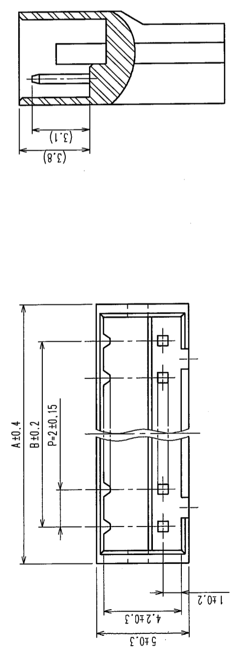
INSERTION FIGURE OF CRIMP CONTACT
