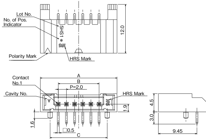
Above drawing is guide-boss type.
