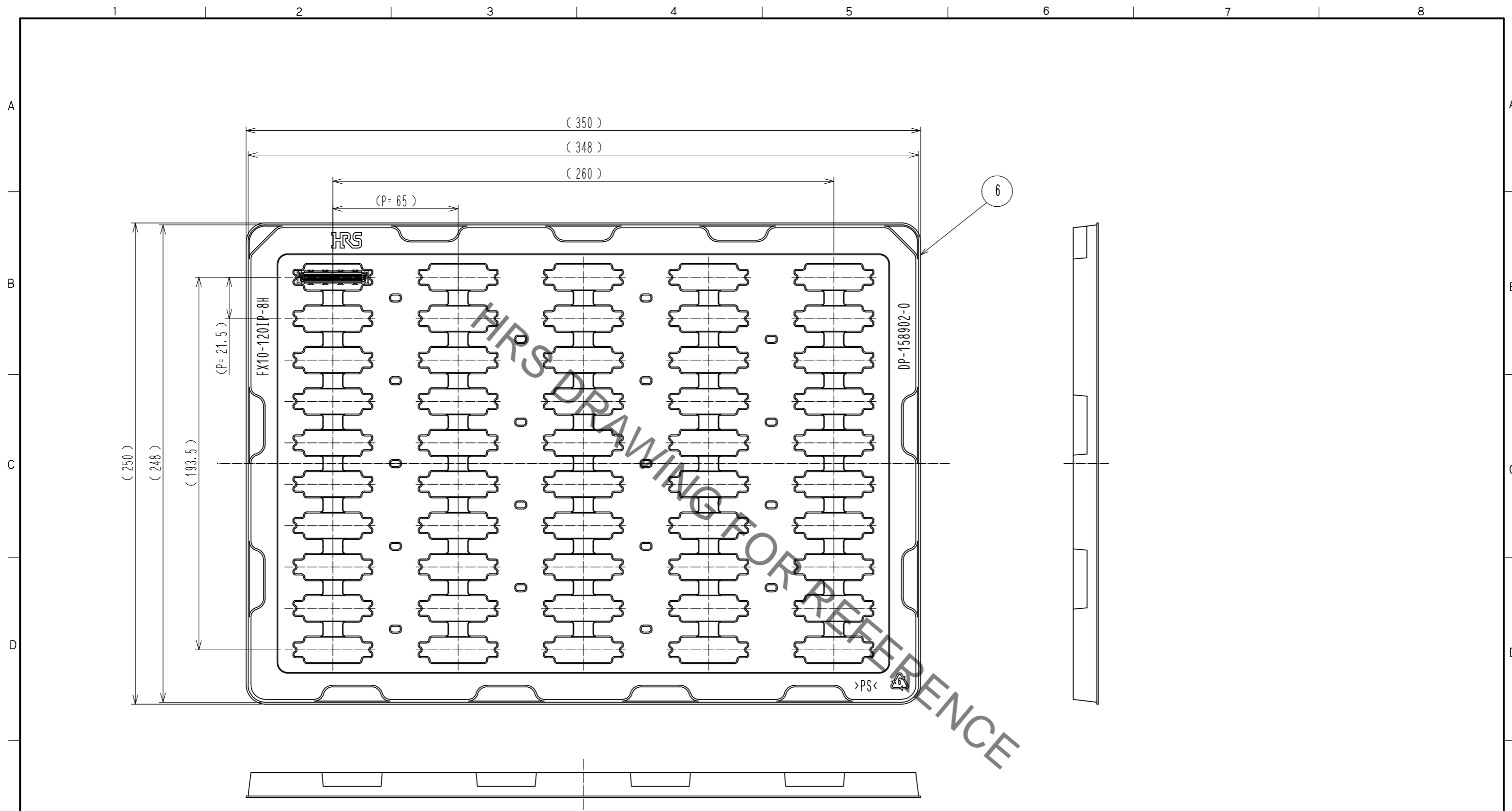
Fig.3 Drawing for packing (1:2) ◁6
