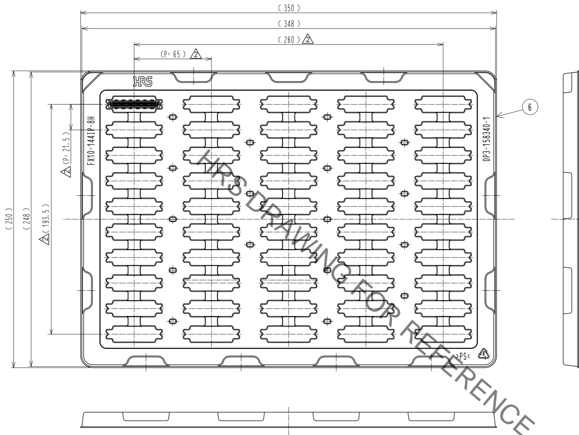
Fig.3 Drawing for packing (1:2) 6
