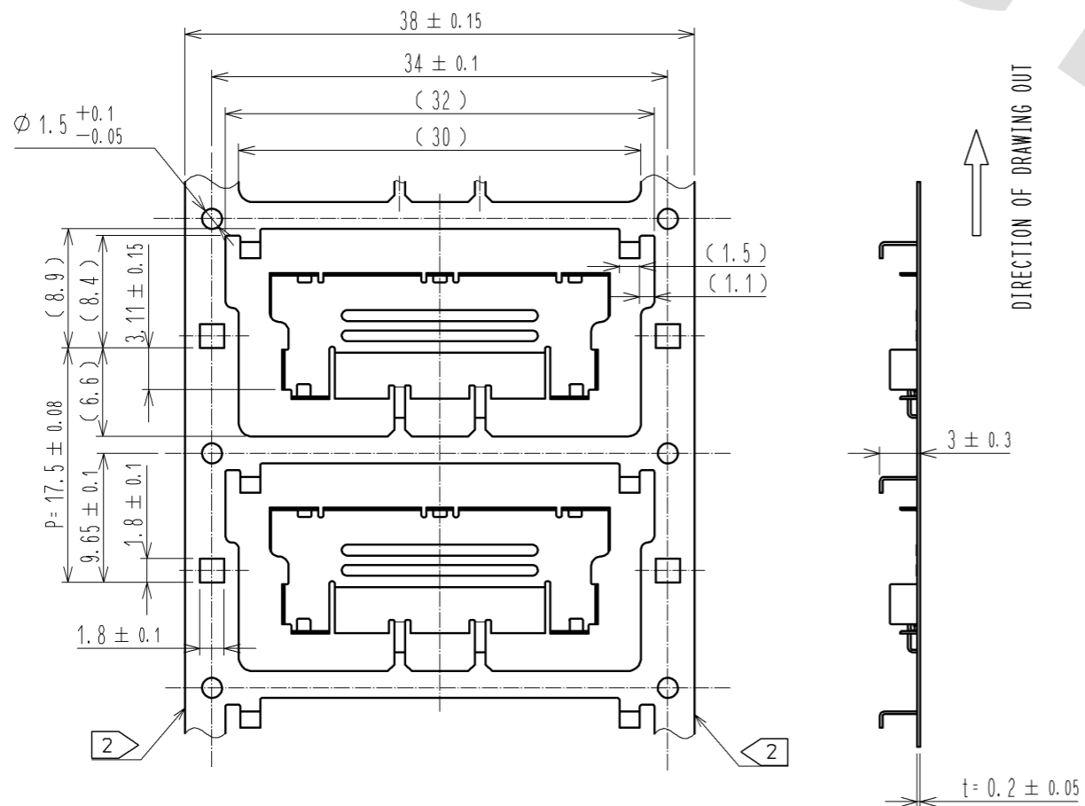
DETAILED FIGURE OF CARRIER (2 : 1)
