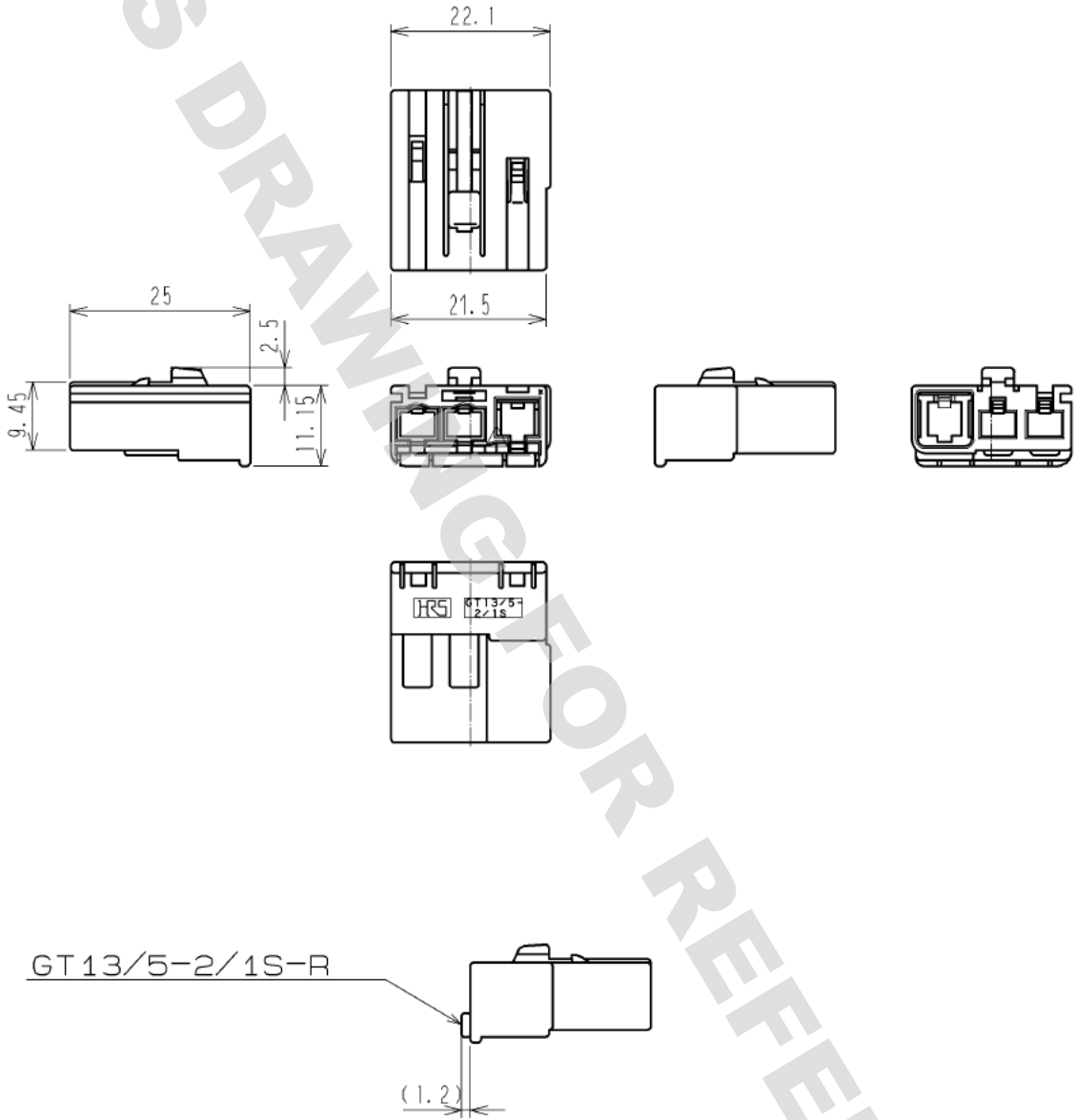
RETAINER ASSEMBLED
