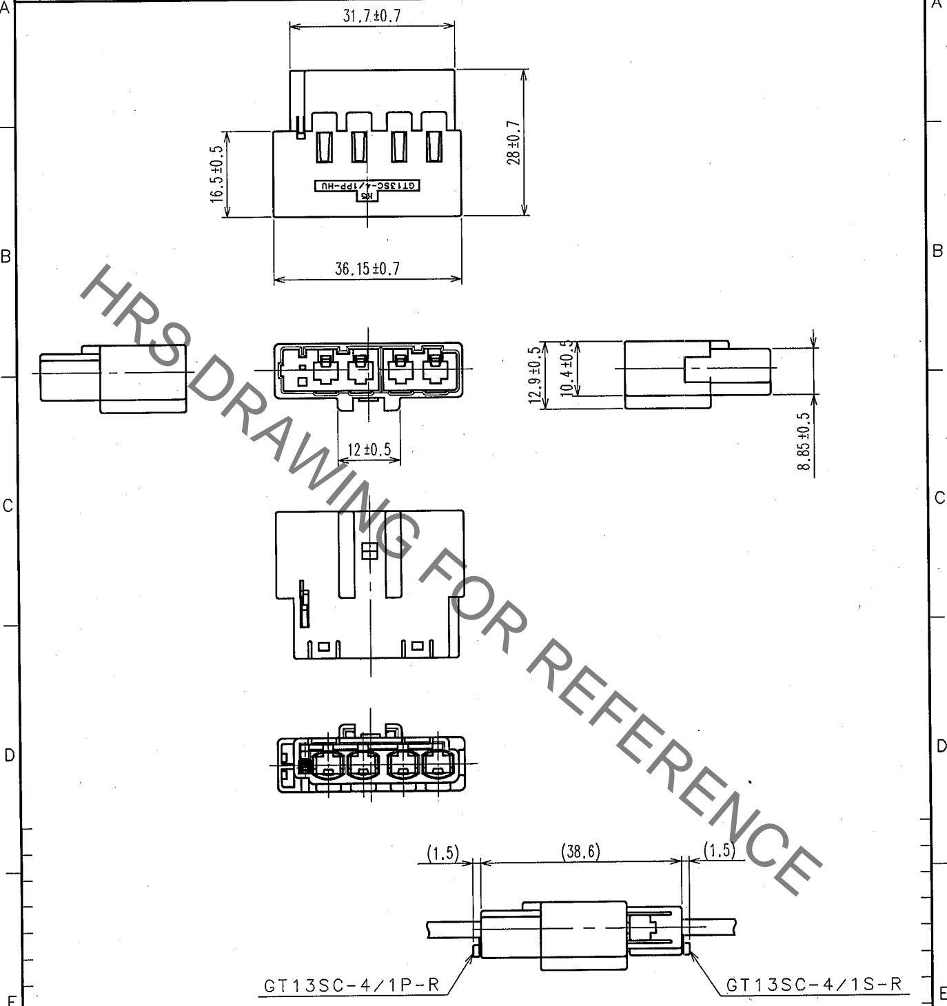
DRAWING WITH RETAINER ATTACHED
