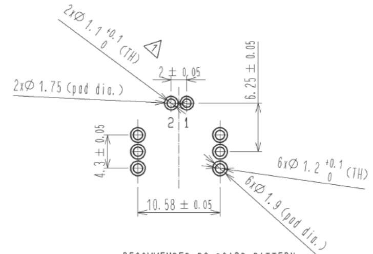
RECOMMENDED PC BOARD PATTERN (CONNECTOR SIDE AND PIN No.)
