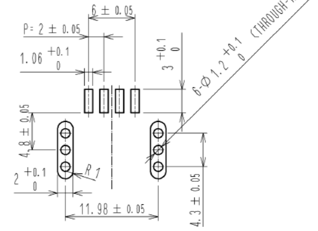
RECOMMENDED PC BOARD PATTERN
