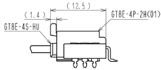
MATING CONFIGURATION
