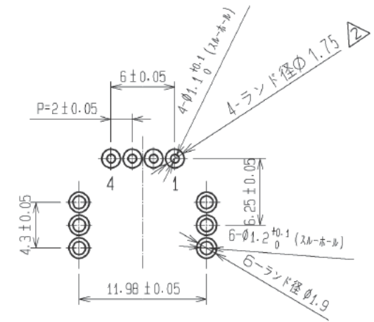
RECOMMENDED PC BOARD PATTERN AND PIN No.
