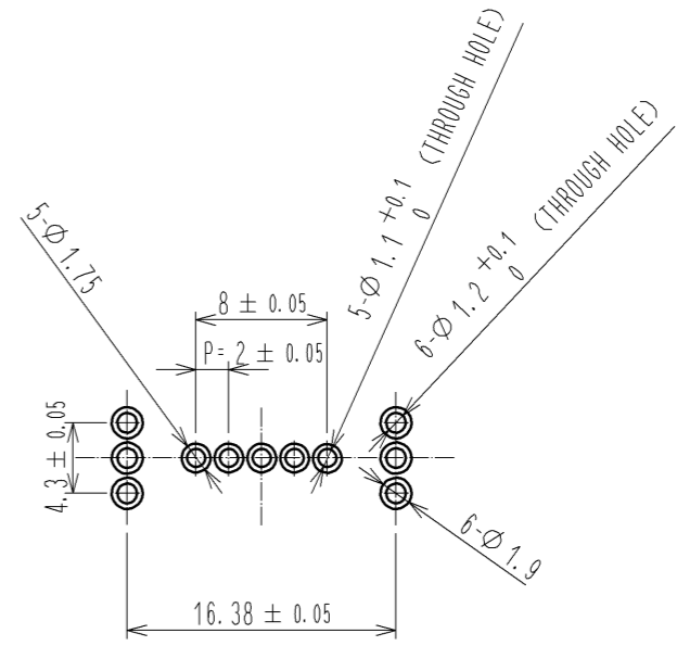
RECOMMENDED PC BOARD PATTERN
