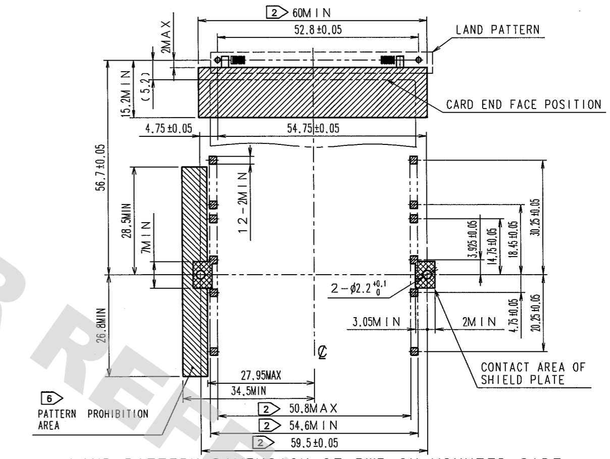
LAND PATTERN DIMENSION OF PWB (ON MOUNTED SIDE) : PATTERN PROHIBITION AREA
