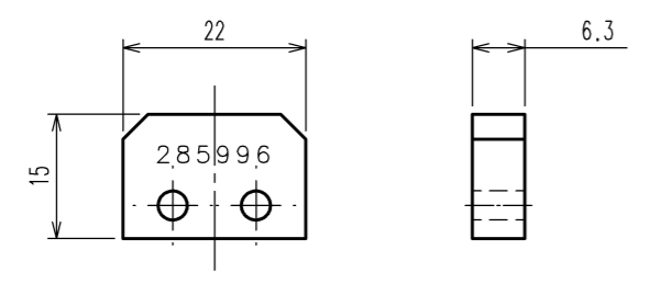
CRIMPER SPACER
