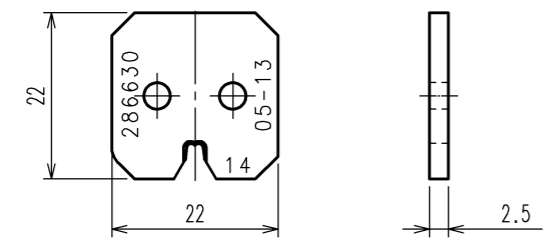
WIRE CRIMPER
