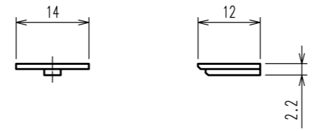
CONTACT HOLDER C
