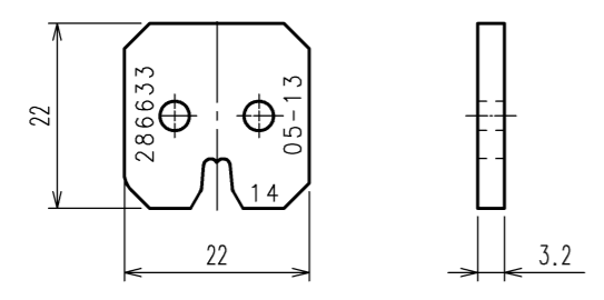
INSULATION CRIMPER
