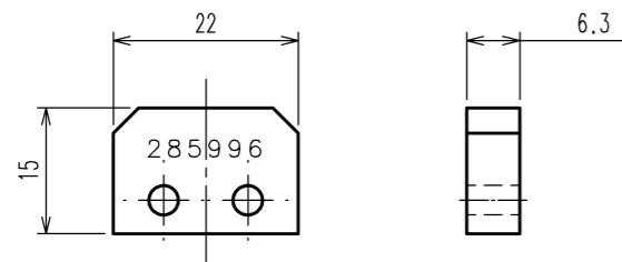
CRIMPER SPACER
