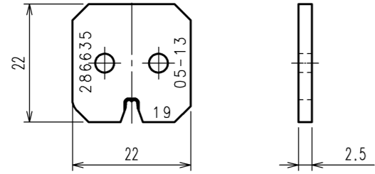
WIRE CRIMPER
