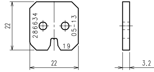
INSULATION CRIMPER
