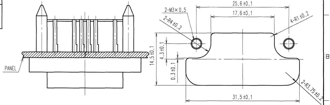
FRONT-MOUNTED
