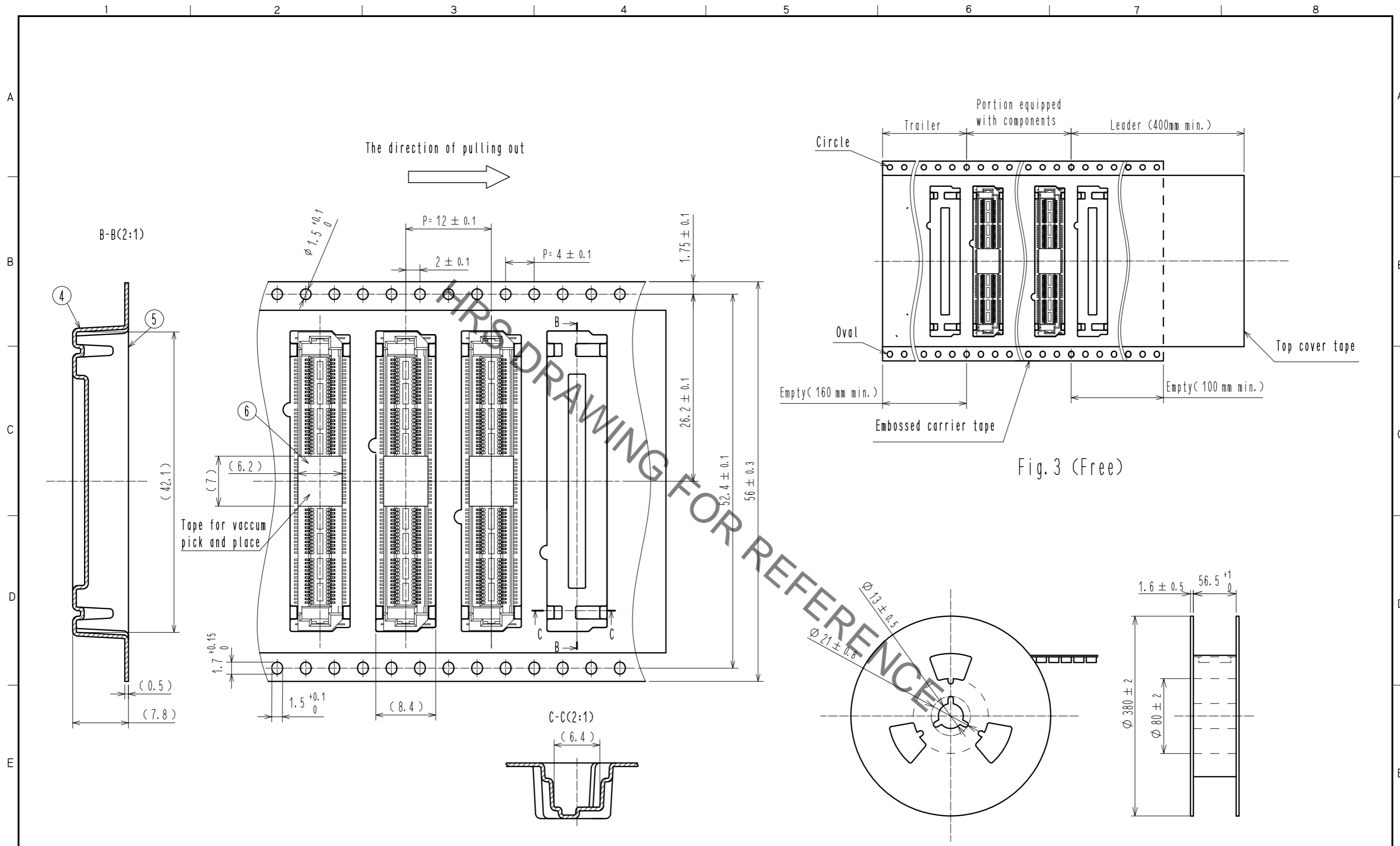
Fig.2 Drawing for packing (2:1)
