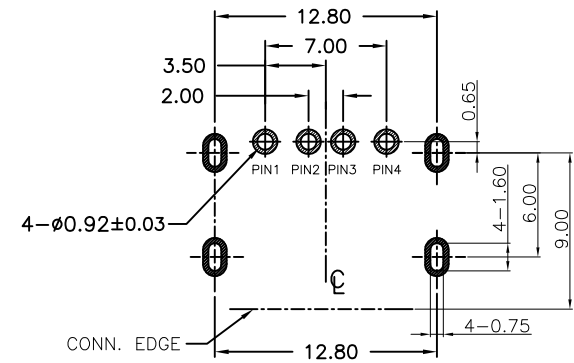
RECOMMENDED PCB LAYOUT(TOP VIEW) GENERAL TOLERANCES:±0.05
